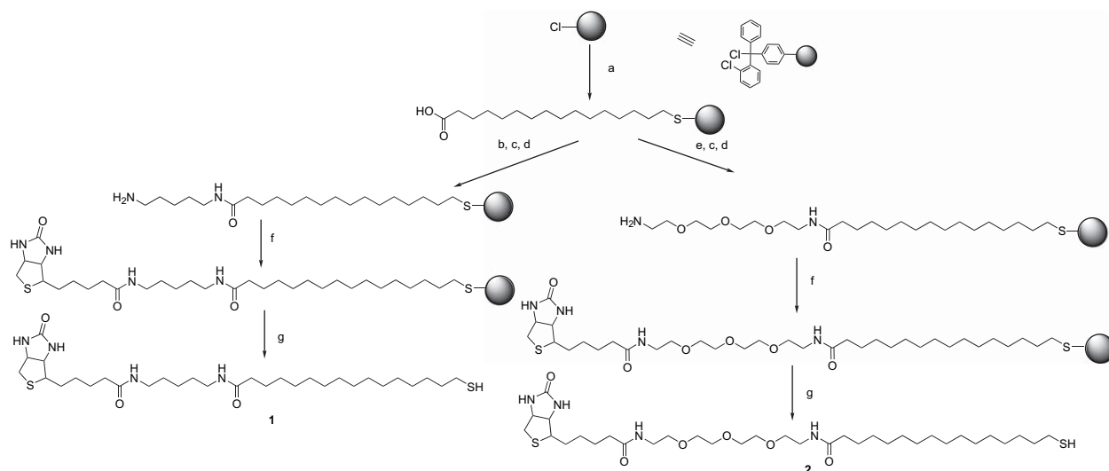
Scheme 1. Solid-phase of 1 and 2 . (a) MHDA (2 equiv), DCM, overnight, rt; (b) Fmoc-diaminopentane hydrochloride (3 equiv), DIPCDI (3 equiv), HOAt (3 equiv), DIPEA (3 equiv), DMF, overnight, rt; (c) MeOH (2 mL/g resin), DIPEA (0.3 mL/g resin), DCM, 10 min, rt; (d) piperidine–DMF (1:4, v/v), 1 × 1 min, 2 × 10 min, rt; (e) Fmoc-1-amino-4,7,10-trioxa-13-tridecanamine hydrochloride (3 equiv), DIPCDI (3 equiv), HOAt (3 equiv), DIPEA (3 equiv), DMF, overnight, rt; (f) Biotin (5 equiv), DICPDI (5 equiv), HOAt (5 equiv), DMF, overnight, rt; (g) TFA 65% in DCM/TES (95:5, v/v).
